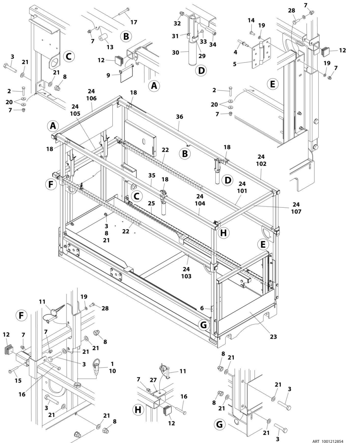
FIGURE 4-7. RAIL (FOLD-DOWN) INSTALLATION WITH EXTENSION HANDLES (6RS/1932RS - CHINA ASSEMBLED MACHINES)
