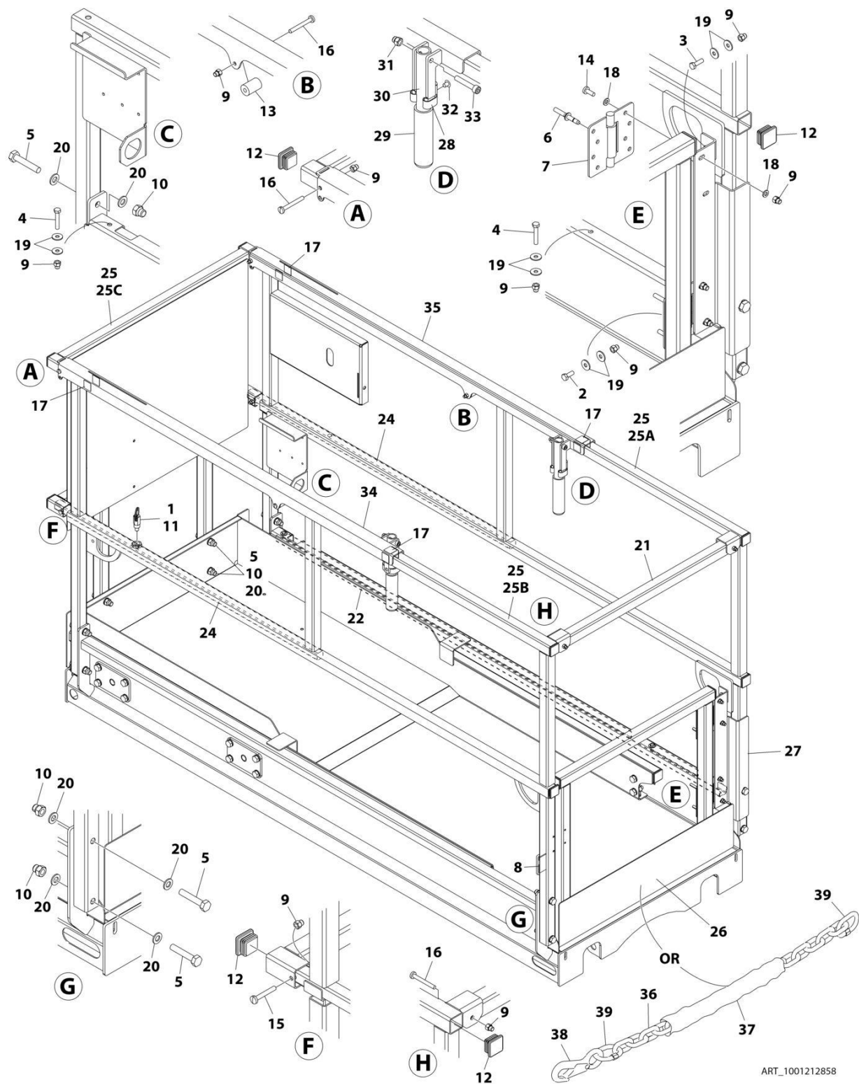
FIGURE 4-4. RAIL (FIXED) INSTALLATION WITH EXTENSION HANDLES (6RS/1932RS - CHINA ASSEMBLED MACHINES)
