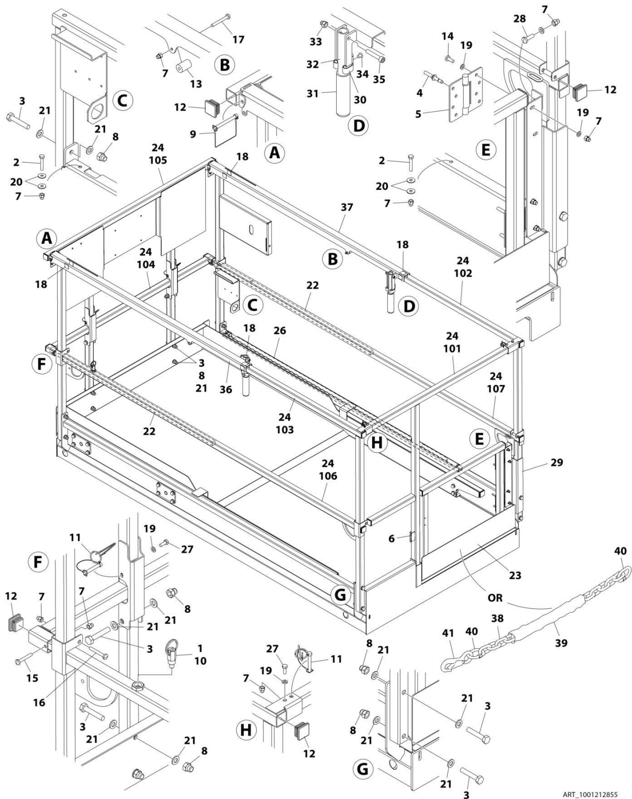
FIGURE 4-9. RAIL INSTALLATION WITH EXTENSION HANDLES (10RS/3248RS - CHINA ASSEMBLED MACHINES)
